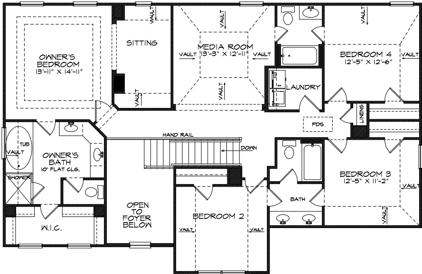
UPPER LEVEL PLAN
