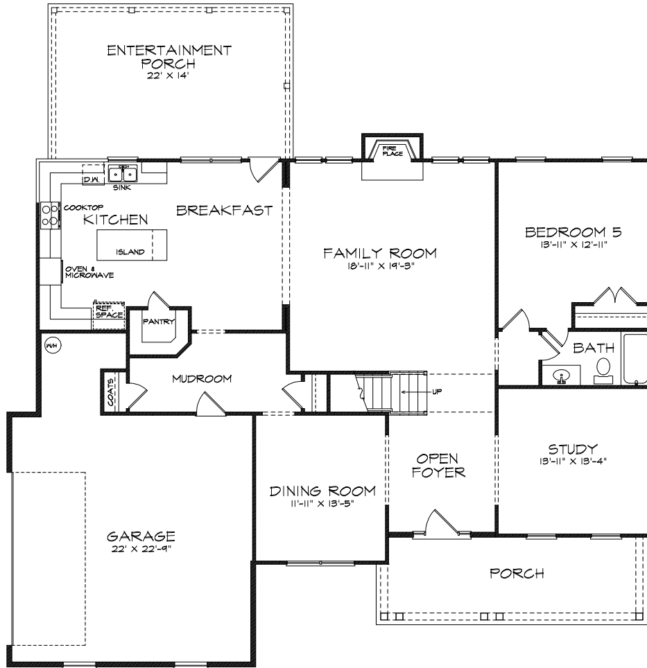
MAIN FLOOR
