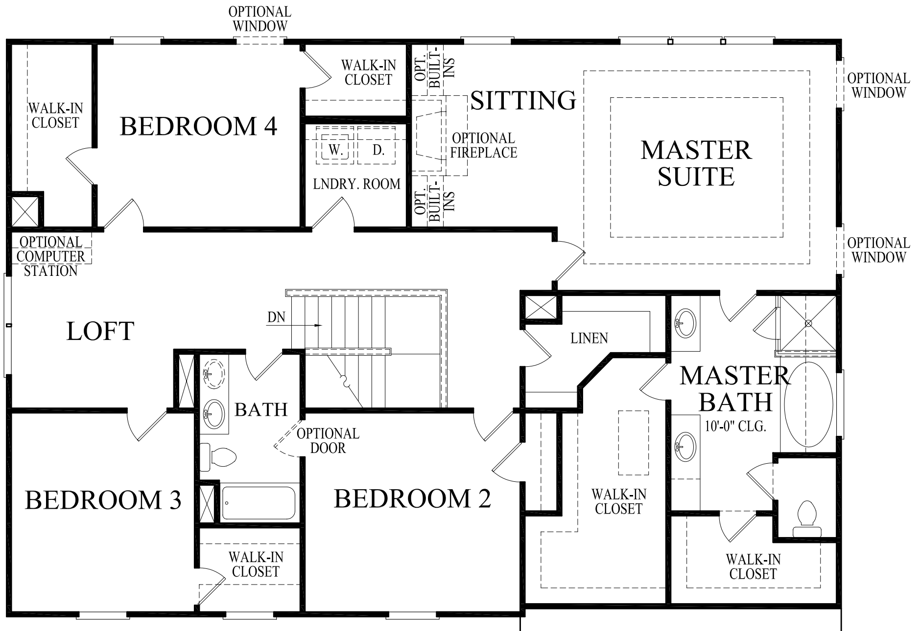
BRIDGEPORT SECOND FLOOR 2-06-09
